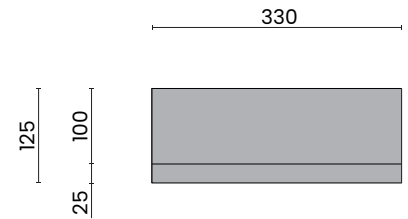
BK1 s (SHORT)
