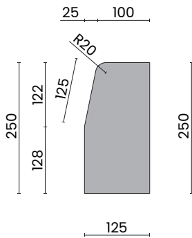
B1 & B1 s SIDE PROFILE
