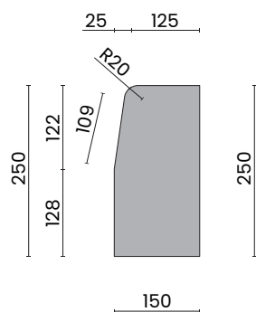
B2 & B2 s SIDE PROFILE
