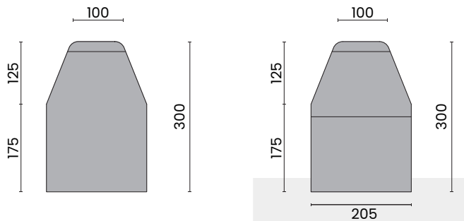
DELINEATOR KERB SIDE PROFILE
