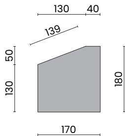
MK10 & MK10 s SIDE PROFILE
