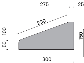
MK4 & MK4 s SIDE PROFILE
