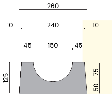
W1 SIDE PROFILE
