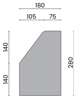
MK2 & MK2 s SIDE PROFILE
